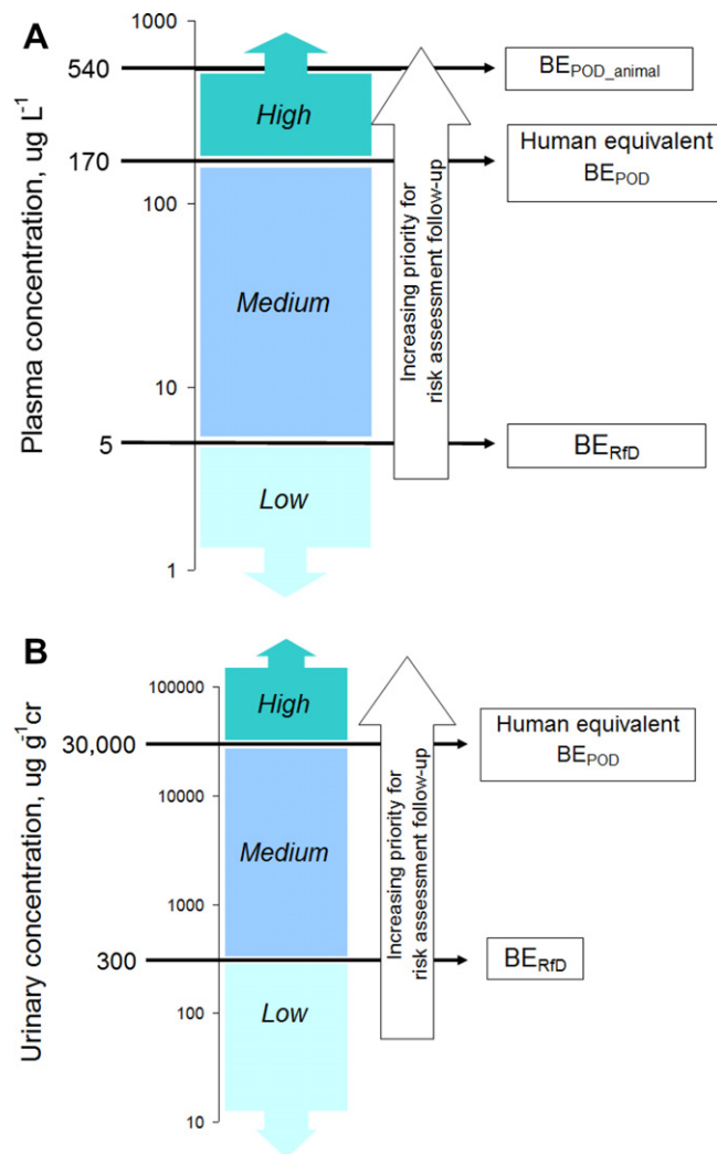
Fig. 3. Guide for interpretation of measured concentrations of 2,4-D in urine or plasma in the context of the chronic BE_{RfD} . Measured concentrations below the BE_{RfD} present a low priority for risk assessment follow-up, while those exceeding that value but below the human equivalent BE_{POD} indicate medium priority, and those in excess of that value suggest high priority. (A) BE values for 2,4-D in plasma; (B) BE values for 2,4-D in urine (creatinine adjusted).
